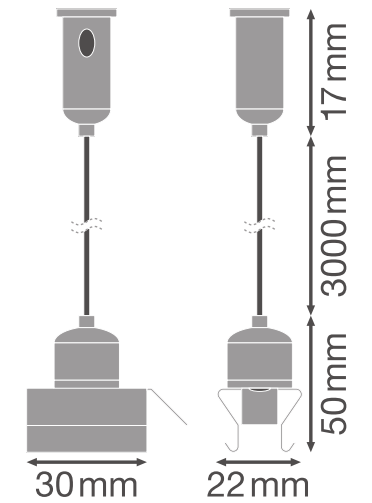
TRUSYS SUSPENSION KIT 3000
