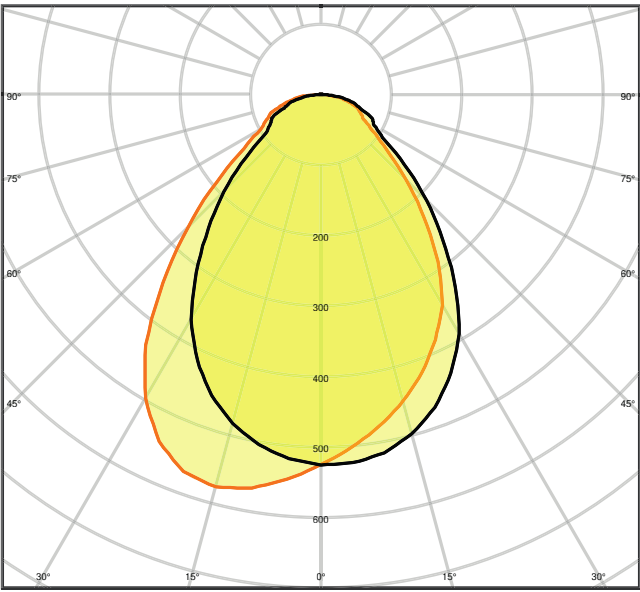
Panel LED 1200 33W 3000K 230V UGR19
