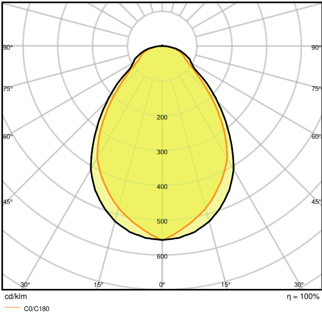
4058075807266 Panel LED 1200 33W 3000K 230V UGR19
