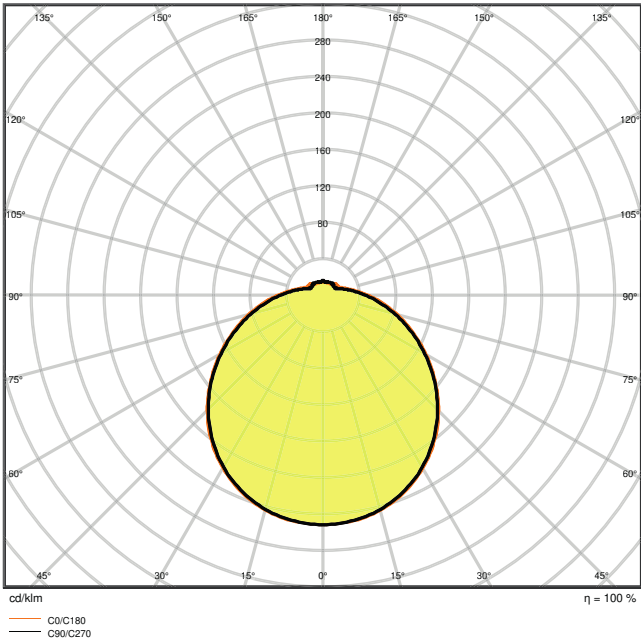
SF CIRCULAR 350 18W 4000K S IP44
